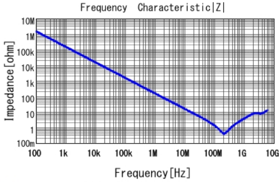
■ GCJ188R71H102KA01 |Z| DCOV, 25degC
