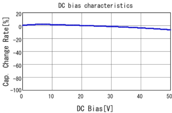
■ GCJ188R71H102KA01 C-DC bias capchange, 25.0degC, AC1.
