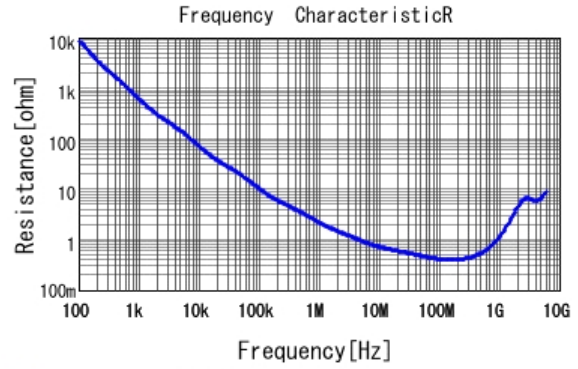
■ GCJ188R71H102KA01 R DCOV, 25degC
