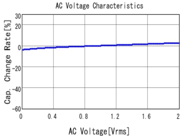
■ GCJ188R71E473KA01 C-AC Voltage capchange, DCOV, 25.0d
