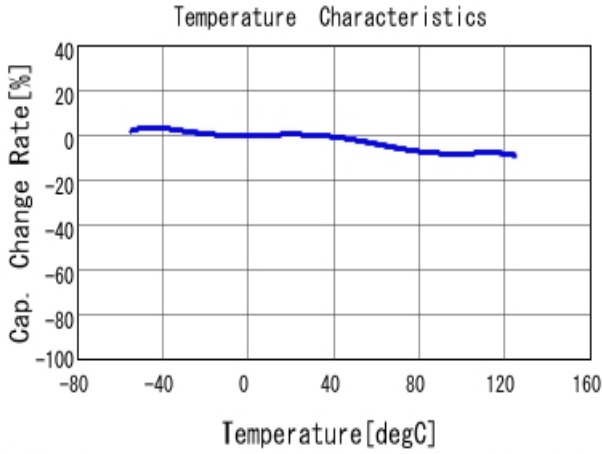
■ GCJ188R71E473KA01 C-Temp. capchange, DC0.0V, AC1.0V rm
