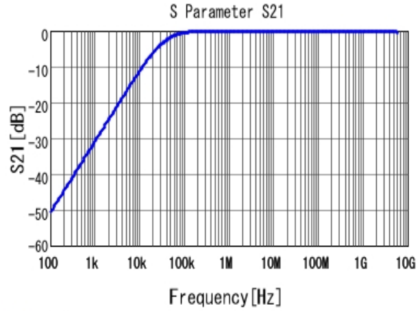
■ GCJ188R71E473KA01 S21 DC0V, 25degC
