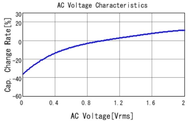
■ GCJ188R71E105KA01 C-AC Voltage capchange, DC0V, 25.0d
