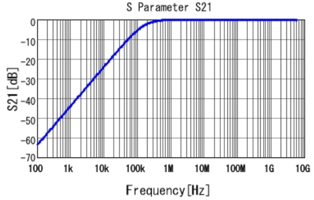
■ GCJ188R71E103KA01 S21 DCOV, 25degC
