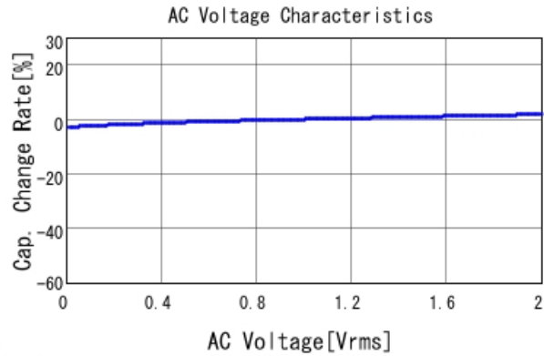
■ GCJ188R71E103KA01 C-AC Voltage capchange, DCOV, 25.0d
