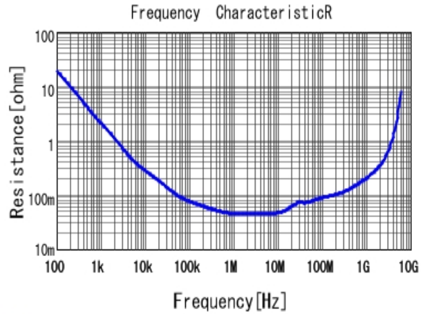
■ GCJ188R71C474KA12 R DC0V, 25degC
