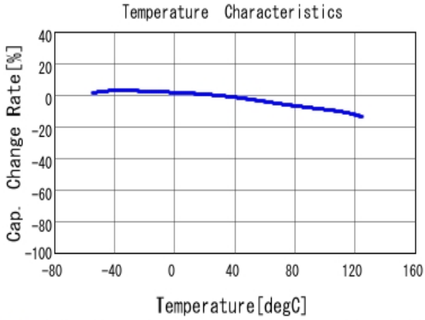
■ GCJ188R71C474KA12 C-Temp. capchange, DC0.0V, AC1.0V r m
