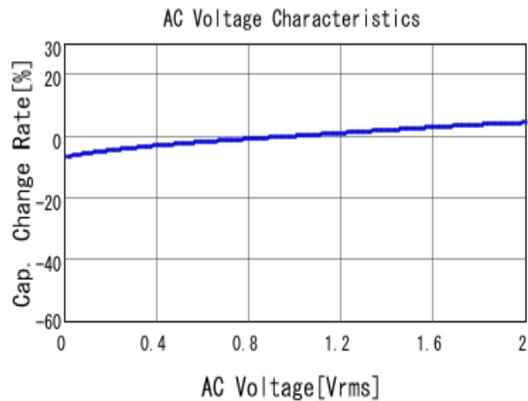
■ GCJ188R71C474KA12 C-AC Voltage capchange, DC0V, 25.0d
