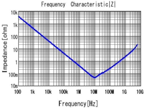
■ GCJ188R71C474KA12 |Z| DC0V, 25degC
