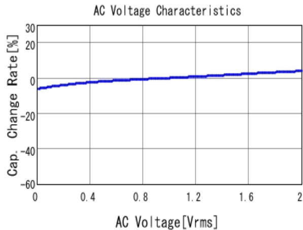
■ GCJ188R71C104KA01 C-AC Voltage capchange, DCOV, 25.0d
