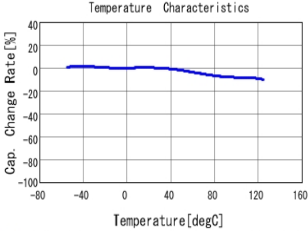
■ GCJ188R71C104KA01 C-Temp. capchange, DC0.0V, AC1.0V rm
