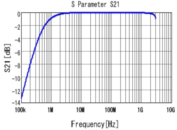
■ GA355QR7GF332KW01 S21 DCOV, 25degC
