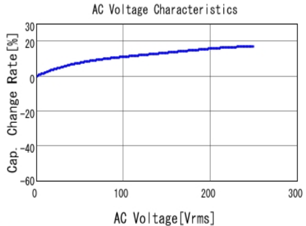
■ GA355QR7GF332KW01 C-AC Voltage capchange, DCOV, 25.0d
