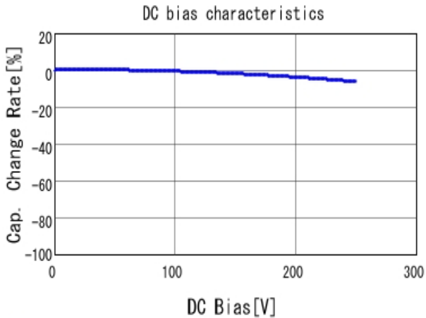
■ GA355QR7GF332KW01 C-DC bias capchange, 25.0degC, AC1V
