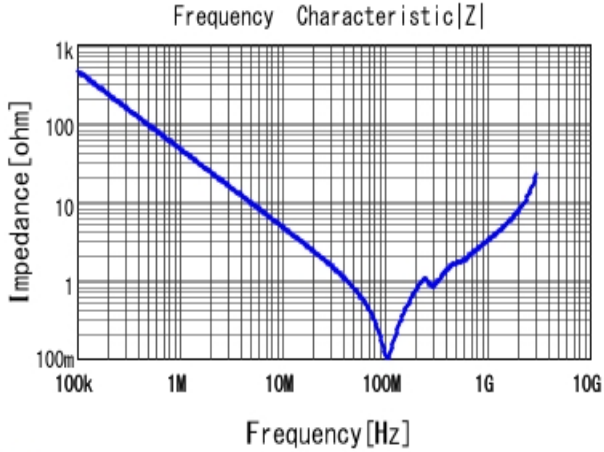
■ GA355QR7GF332KW01 |Z| DCOV, 25degC
