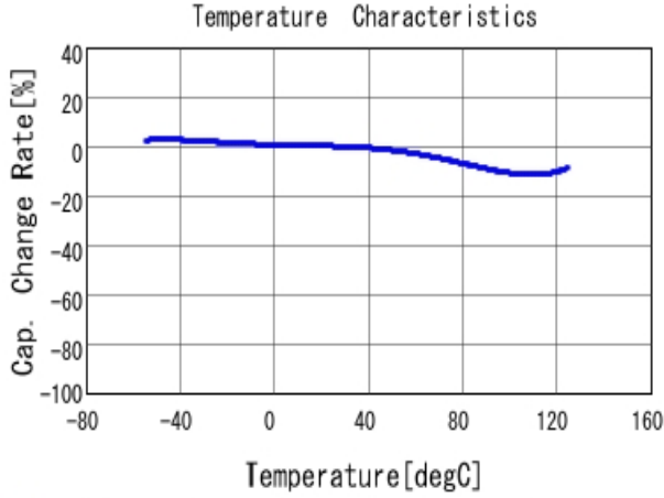
■ GA355QR7GF332KW01 C-Temp. capchange, DCOV, AC1Vrms
