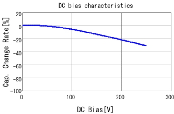
■ GA355ER7GB473KW01 C-DC bias capchange, 25.0degC, AC1V
