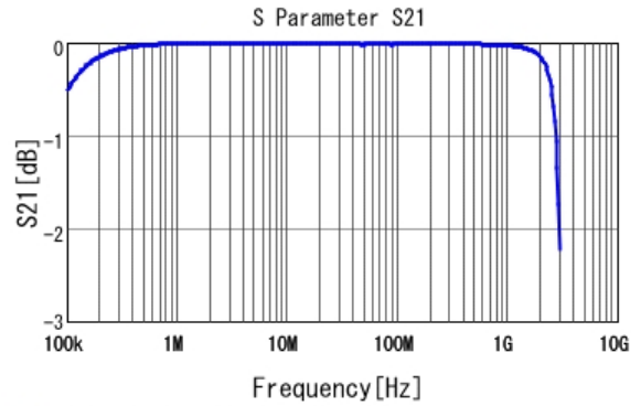
■ GA355ER7GB473KW01 S21 DC0V, 25degC
