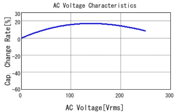
■ GA355ER7GB473KW01 C-AC Voltage capchange, DC0V, 25.0d
