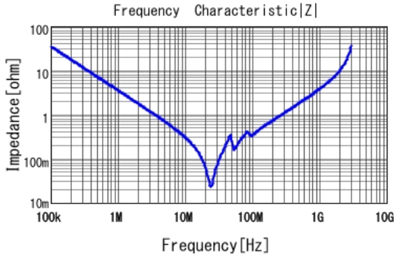
■ GA355ER7GB473KW01 |Z| DC0V, 25degC
