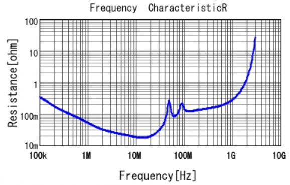
■ GA355ER7GB473KW01 R DC0V, 25degC
