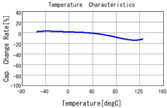
■ GA355ER7GB473KW01 C-Temp. capchange, DC0V, AC1Vrms
