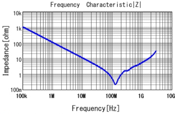
■ GA352QR7GF152KW01 |Z| DCOV, 25degC
