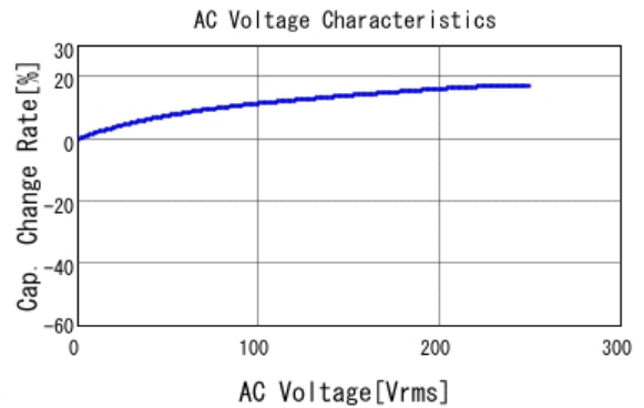
■ GA352QR7GF152KW01 C-AC Voltage capchange, DCOV, 25.0d
