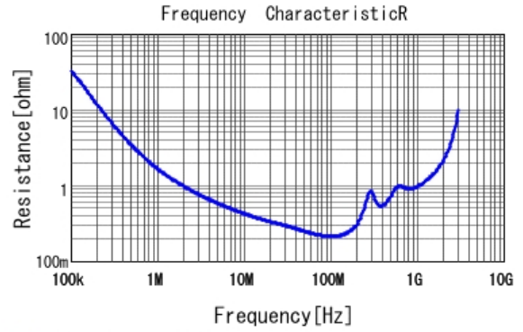
■ GA352QR7GF152KW01 R DCOV, 25degC
