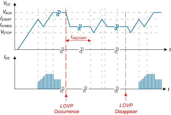
Figure 25. LOVP Waveforms
