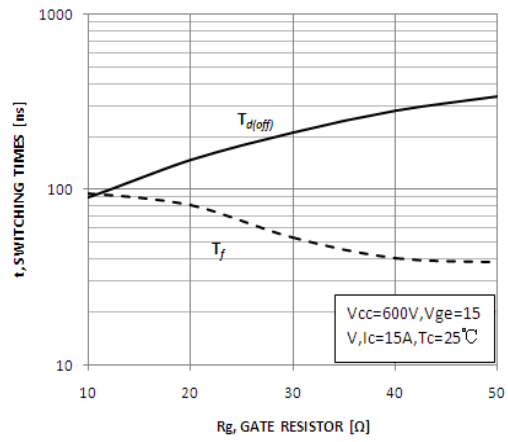
Figure 8. Typical Turn-Off Characteristics vs. Gate Resistance
