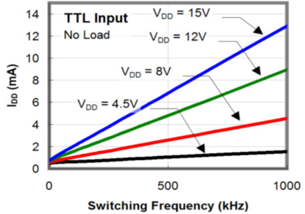
Figure 14. I DD (No-Load) vs. Frequency
