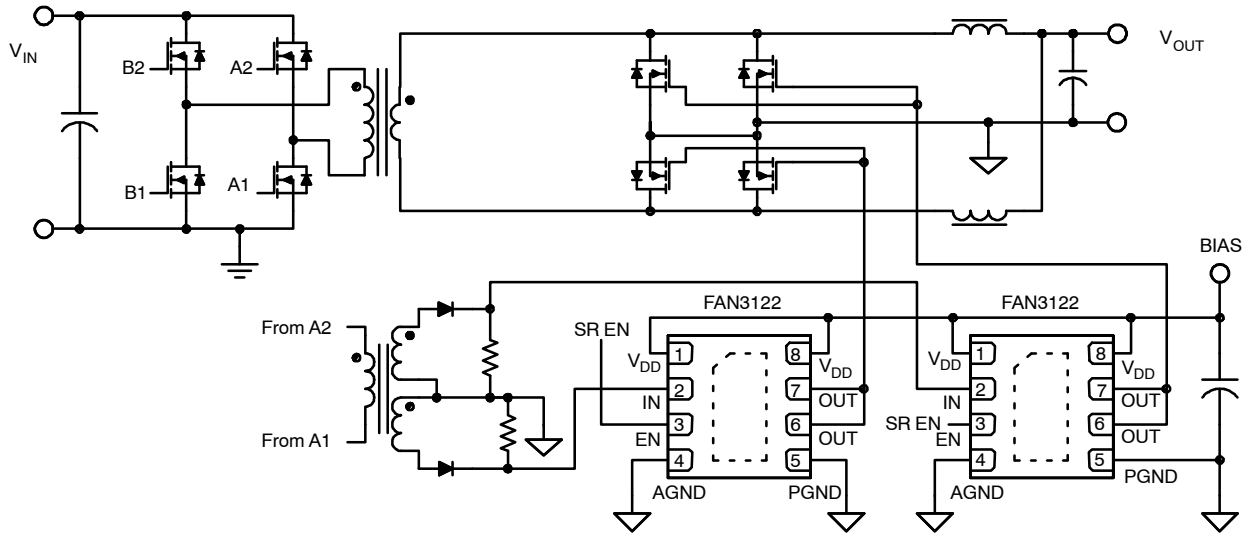
Figure 54. Full-Bridge Synchronous Rectification
