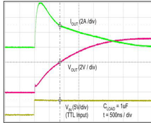
Figure 44. Quasi-Static Source Current with VDD = 8 V (Note 14)
