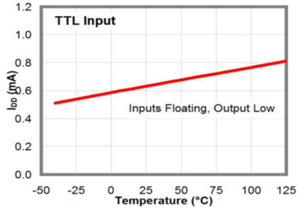
Figure 18. I DD (Static) vs. Temperature (Note 13)
