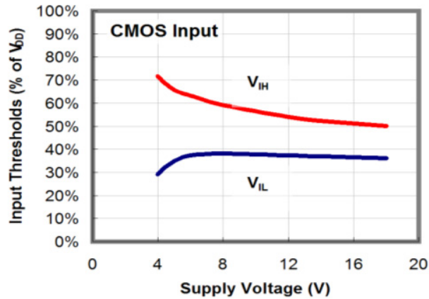
Figure 21. Input Thresholds % vs. Supply Voltage
