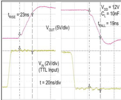
Figure 41. Rise / Fall Waveforms with 10 nF Load
