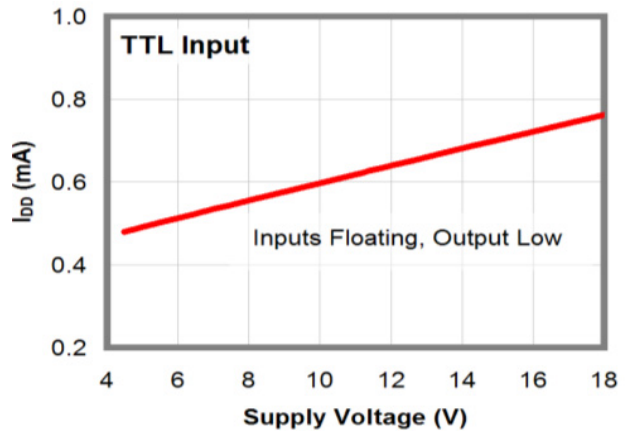
Figure 12. I DD (Static) vs. Supply Voltage (Note 13)
