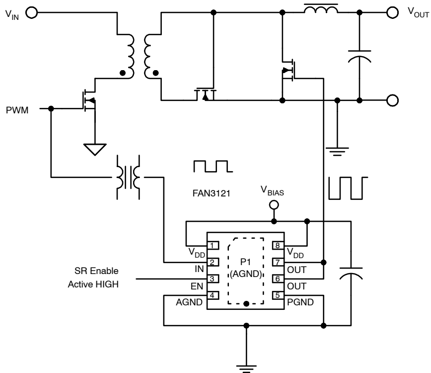
Figure 55. Hybrid Synchronous Rectification in a Forward Converter
