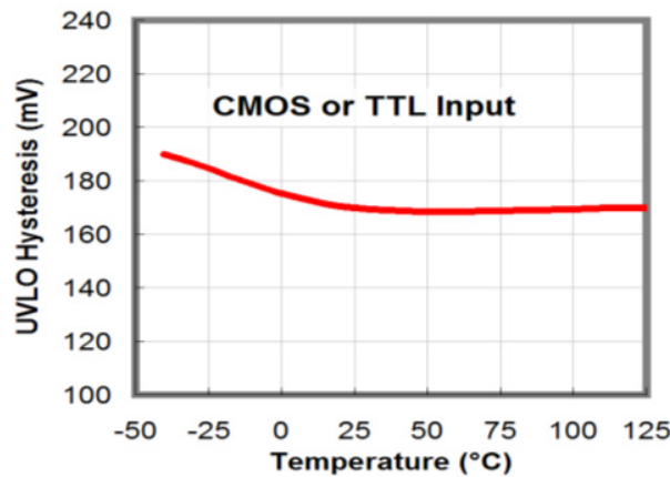
Figure 27. UVLO Hysteresis vs. Temperature
