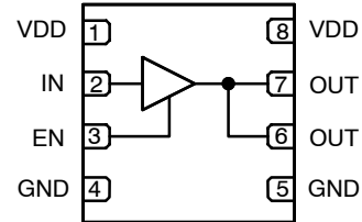
Figure 7. FAN3122 Pin Assignments (Repeated)
