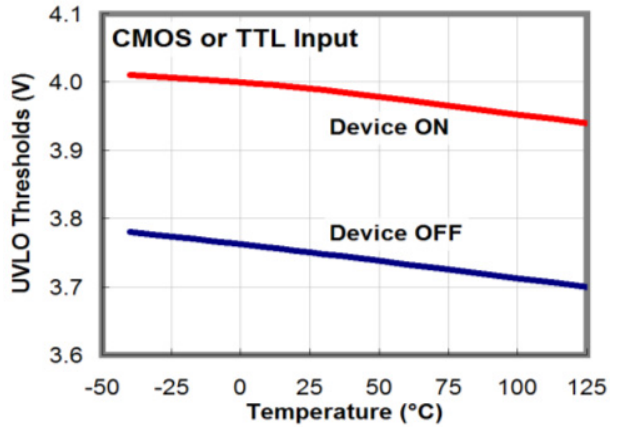
Figure 26. UVLO Thresholds vs. Temperature
