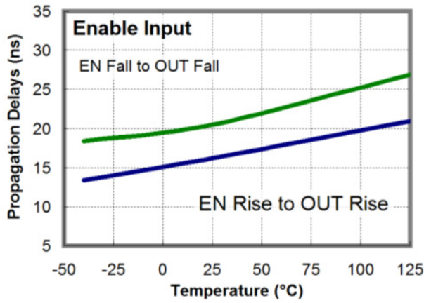
Figure 37. Propagation Delays vs. Temperature
