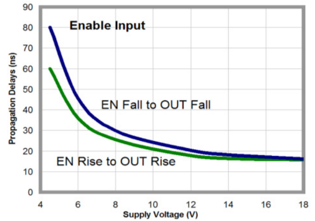
Figure 32. Propagation Delay vs. Supply Voltage
