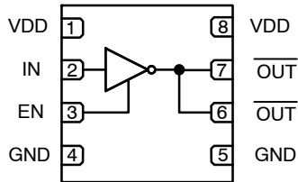
Figure 6. FAN3121 Pin Assignments (Repeated)
