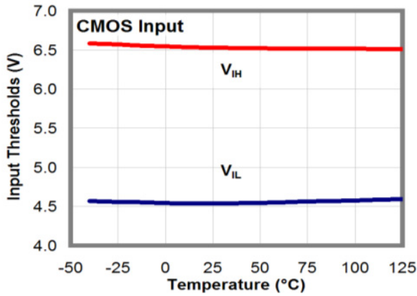
Figure 23. CMOS Input Thresholds vs. Temperature
