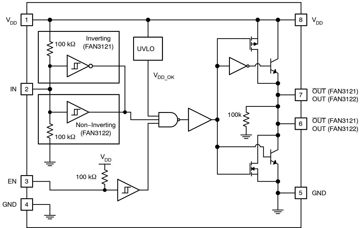
Figure 8. Block Diagram
