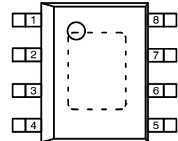
Figure 5. SOIC-8-EP (Top View)
