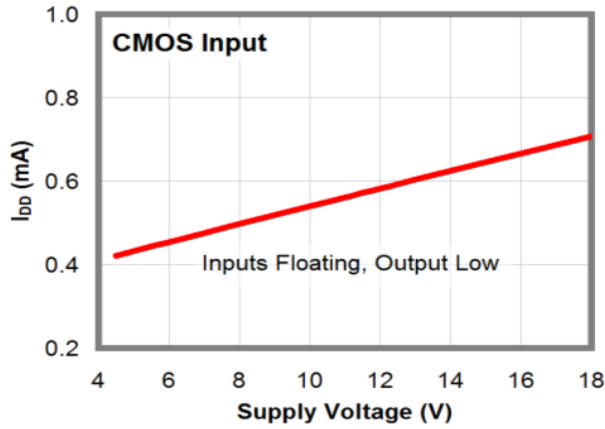
Figure 11. I DD (Static) vs. Supply Voltage (Note 13)
