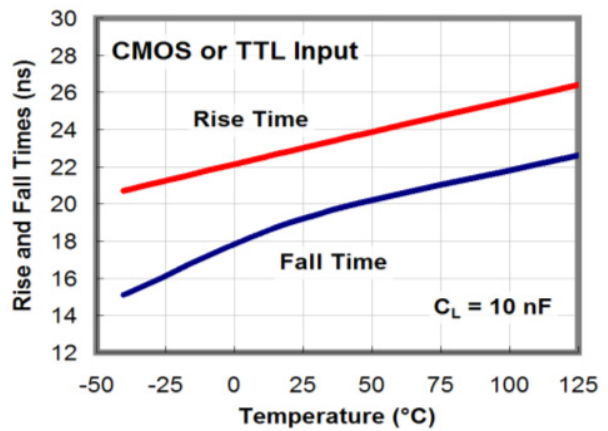
Figure 40. Rise and Fall Time vs. Temperature
