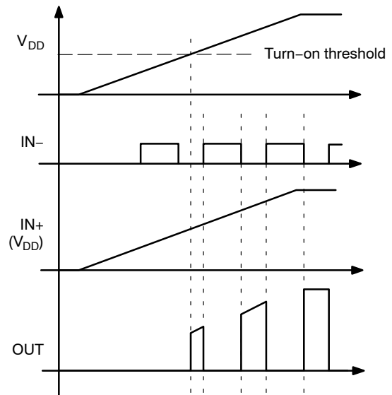
Figure 51. Inverting Startup Waveforms
