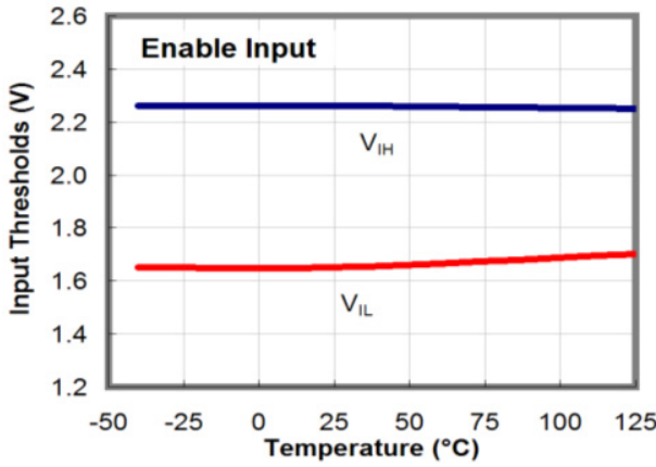
Figure 25. TTL Input Thresholds vs. Temperature
