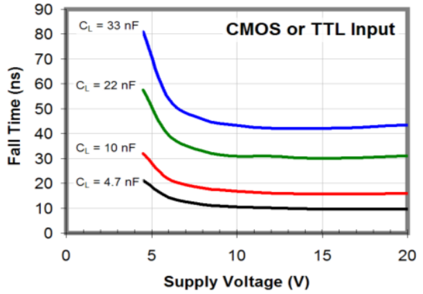
Figure 38. Fall Time vs. Supply Voltage
