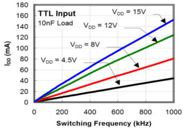
Figure 16. I DD (10 nF Load) vs. Frequency
