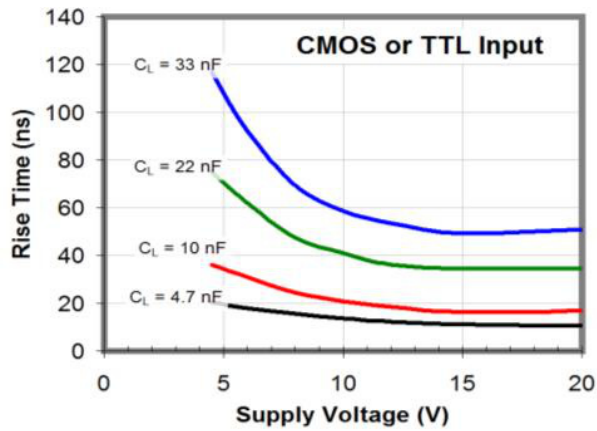
Figure 39. Rise Time vs. Supply Voltage
