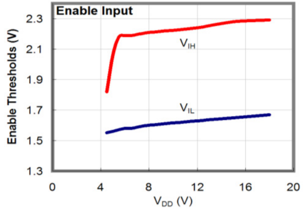
Figure 22. Enable Thresholds vs. Supply Voltage
