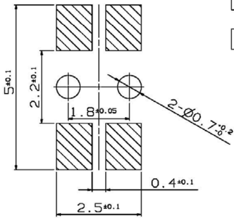
Land pattern plan
