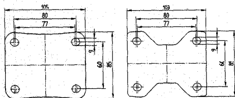
Swivel Castor P 62-105x85
