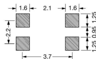
Figure 2) Suggested land pattern
