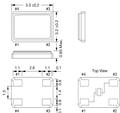
Figure 1) Top, Side, and Bottom
