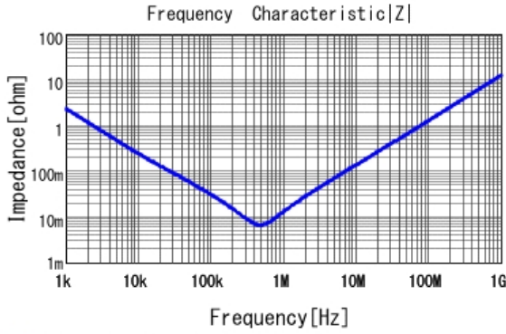
■ ECASD61A686M015K00 |Z| DCOV, 25degC
