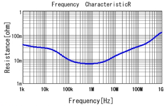
■ ECASD61A686M015K00 R DCOV, 25degC
