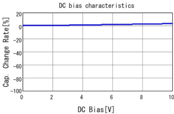
■ ECASD61A686M015K00 C-DC bias capchange, 25.0degC, AC1
