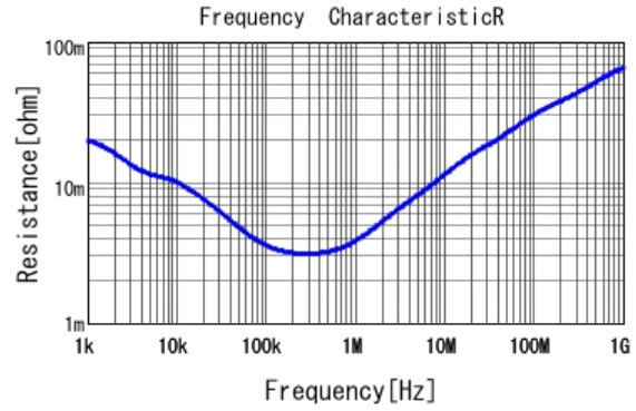
■ ECASD60J227M010K00 R DCOV, 25degC
