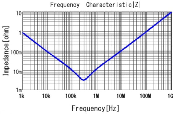
■ ECASD60J227M010K00 |Z| DCOV, 25degC
