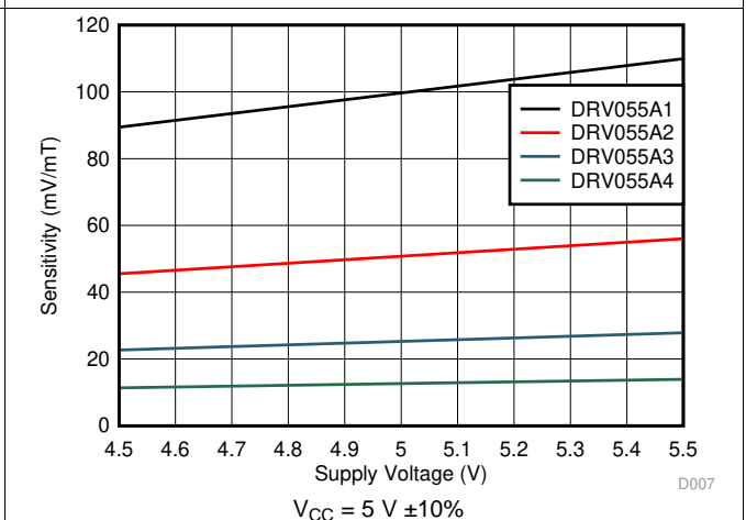
Figure 10. Sensitivity vs Supply Voltage
