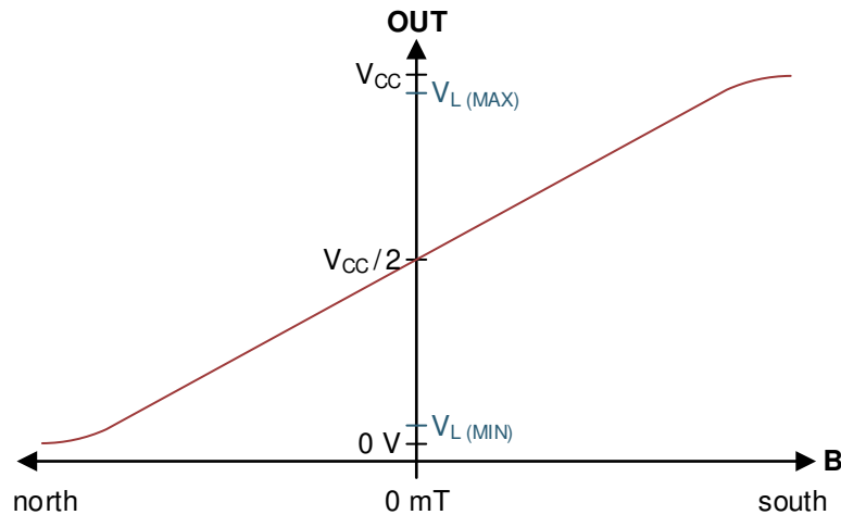
Figure 16. Magnetic Response
