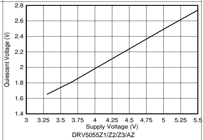
Figure 4. Quiescent Voltage vs Supply Voltage
