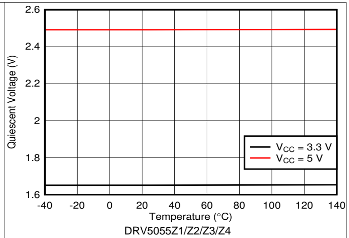
Figure 2. Quiescent Voltage vs Temperature
