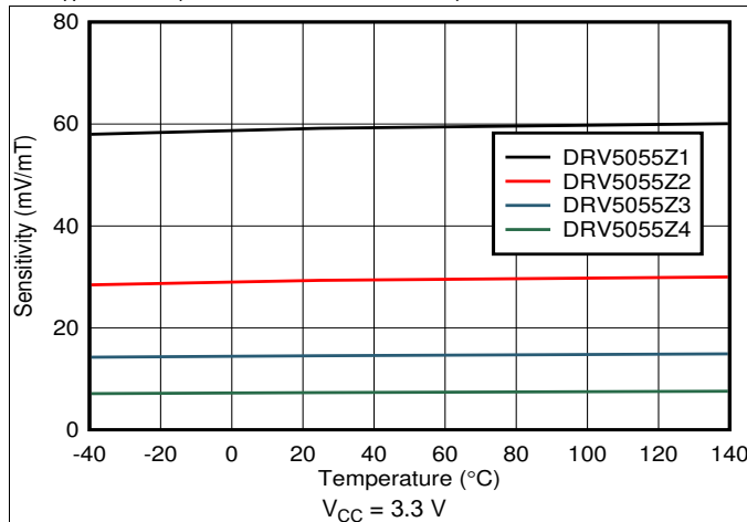
Figure 7. Sensitivity vs Temperature
