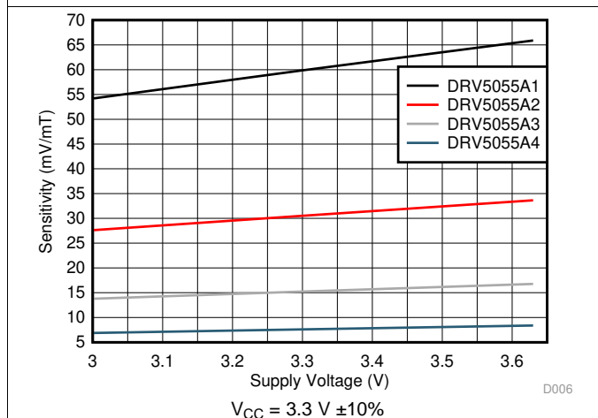
Figure 9. Sensitivity vs Supply Voltage
