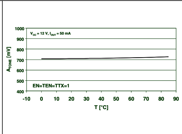
Figure 21. Tone amplitude vs. temperature
