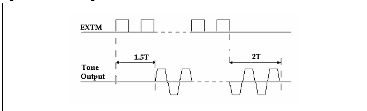
Figure 2. EXTM timings
