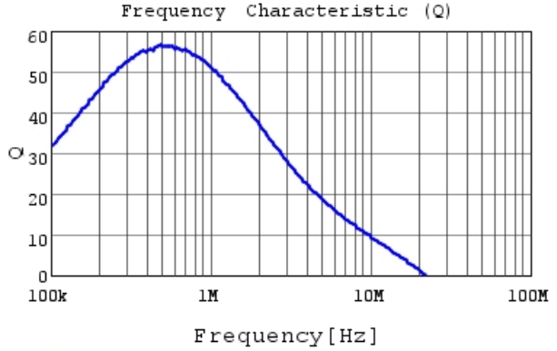
DFE322520FD-4R7M Q
