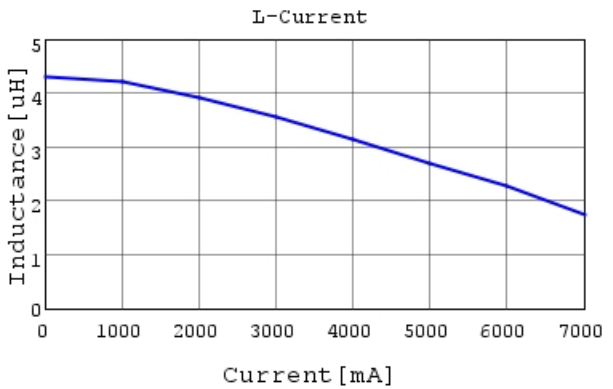
DFE322520FD-4R7M L-Current 20degC
