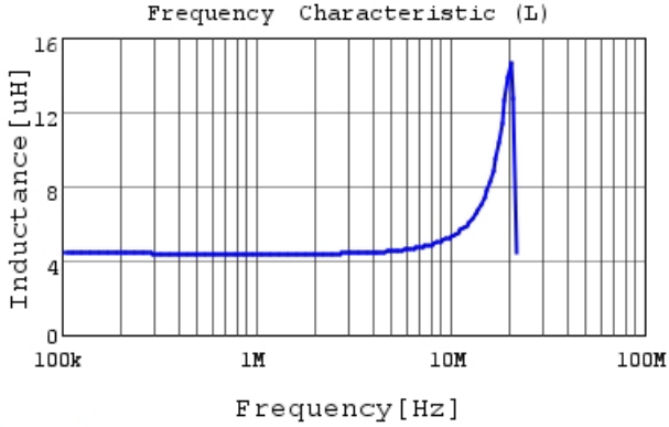
DFE322520FD-4R7M L
