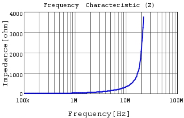
DFE322520FD-4R7M |Z|
