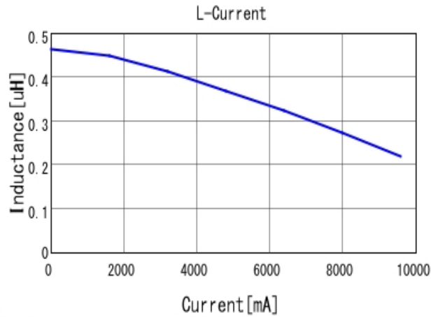
DFE252012P-R47M L-Current 20degC
