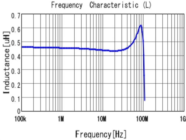
DFE252012P-R47M L
