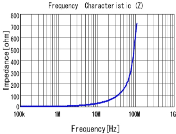
DFE252012P-R47M |Z|
