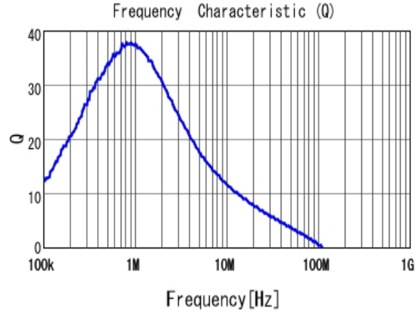
DFE252012P-R47M Q
