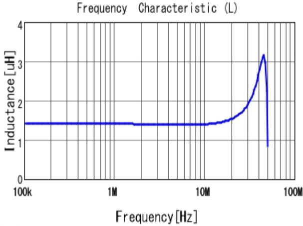
DFE252012P-1R5M L
