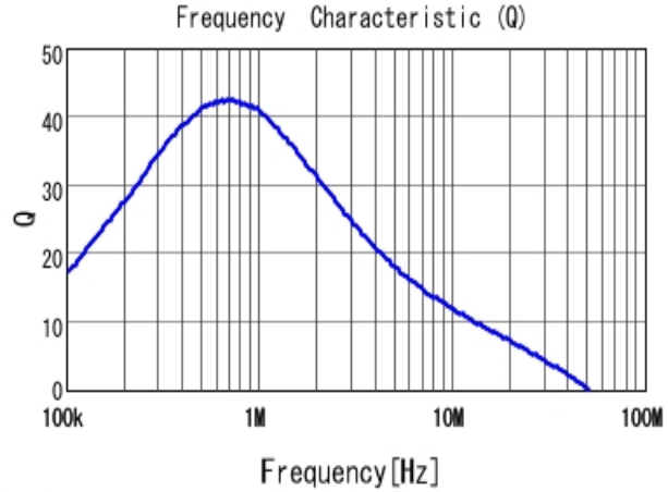
DFE252012P-1R5M Q
