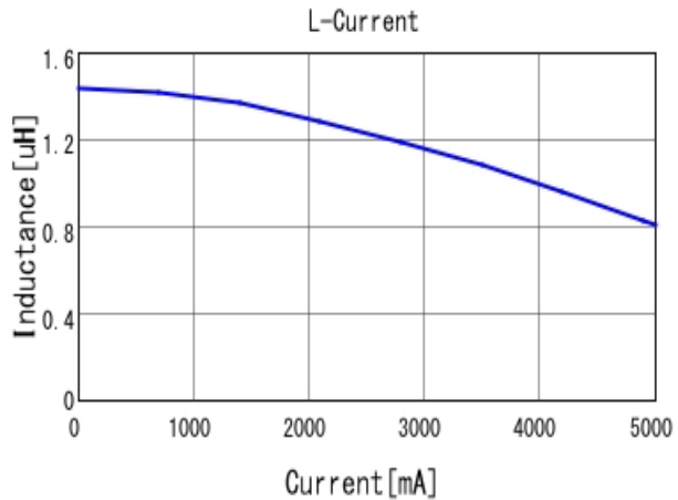
DFE252012P-1R5M L-Current 20degC
