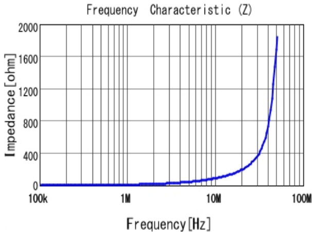
DFE252012P-1R5M |Z|
