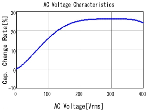
■ DE2E3SA222MA3BY02F C-AC Voltage capchange, DCOV, 20.0
