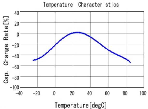
■ DE2E3SA222MA3BY02F C-Temp. capchange, DCOV, AC1Vrms
