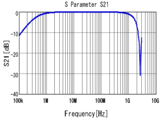
■ DE2E3KY472MN2AM01F S21 DCOV, 20degC
