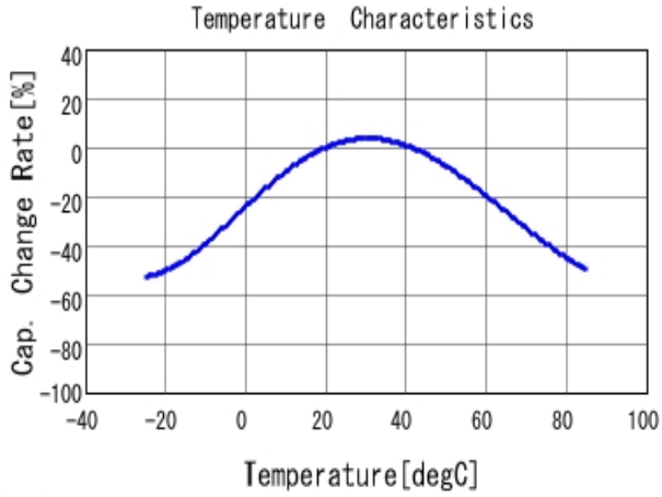
■ DE2E3KY472MN2AM01F C-Temp. capchange, DCOV, AC1Vrms
