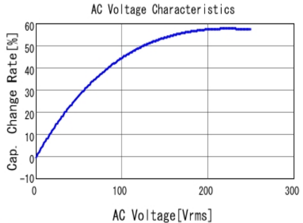
■ DE2E3KY472MN2AM01F C-AC Voltage capchange, DC0V, 20.0
