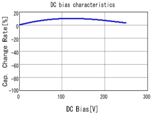
■ DE2E3KY472MN2AM01F C-DC bias capchange, 20.0degC, AC1
