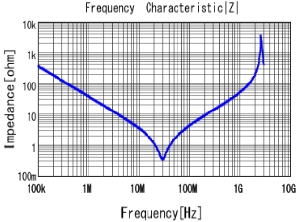
■ DE2E3KY472MN2AM01F |Z| DC0V, 20degC
