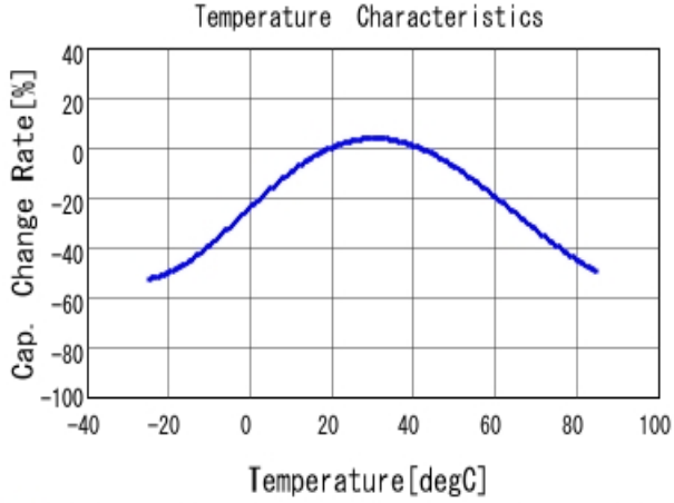
■ DE2E3KY222MB2BM01F C-Temp. capchange, DCOV, AC1Vrms
