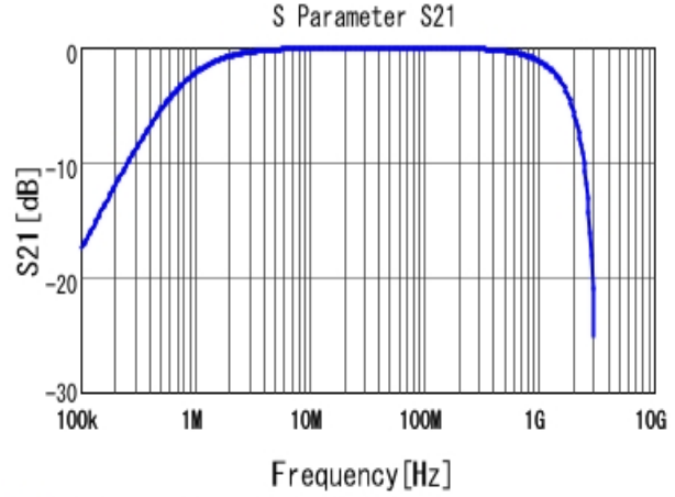
■ DE2E3KY222MB2BM01F S21 DCOV, 20degC
