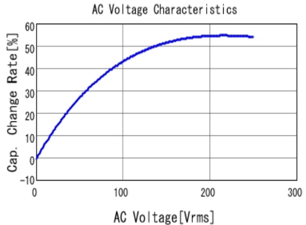
■ DE2E3KY222MB2BM01F C-AC Voltage capchange, DCOV, 20.0
