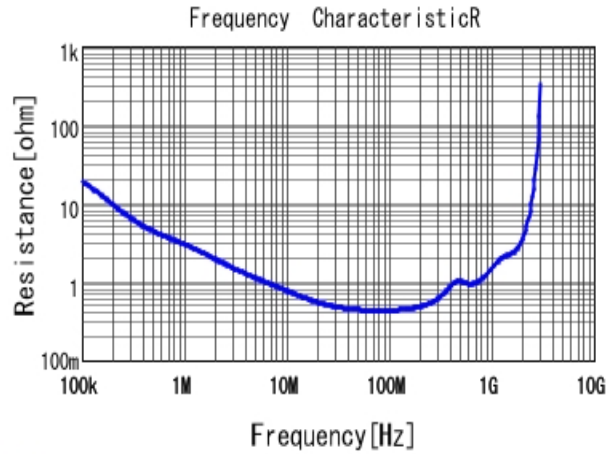
■ DE2E3KY222MB2BM01F R DCOV, 20degC
