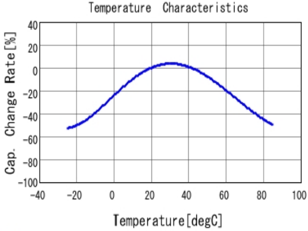
■ DE2E3KY102MN2AM01F C-Temp. capchange, DCOV, AC1Vrms
