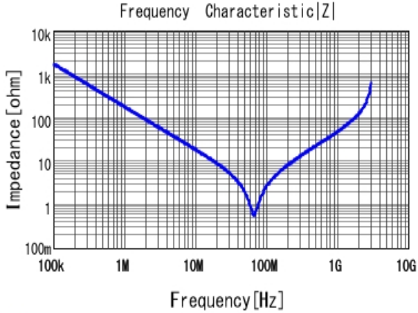
■ DE2E3KY102MN2AM01F |Z| DCOV, 20degC
