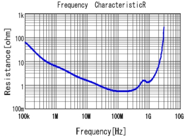
■ DE2E3KY102MN2AM01F R DCOV, 20degC
