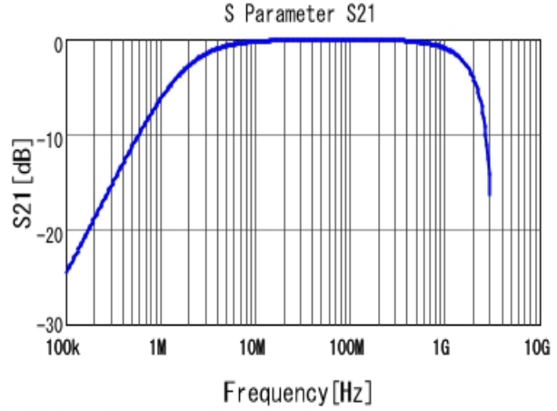
■ DE2E3KY102MN2AM01F S21 DCOV, 20degC
