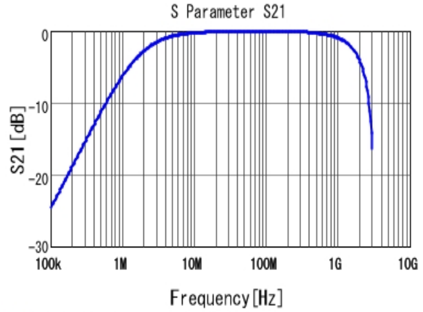
■ DE2E3KY102MB3BM02F S21 DCOV, 20degC
