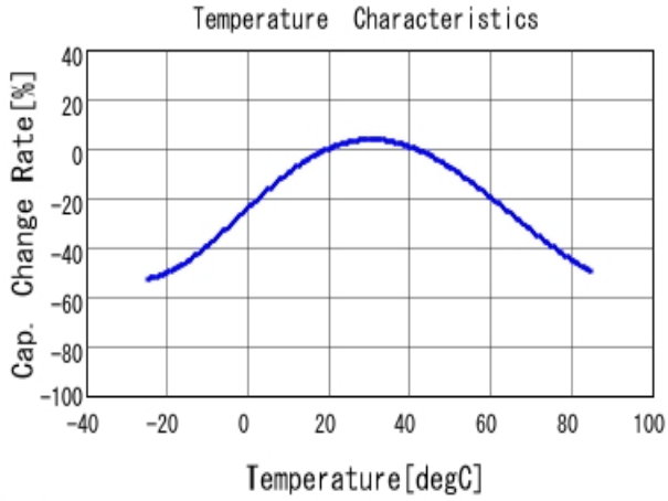
■ DE2E3KY102MB3BM02F C-Temp. capchange, DCOV, AC1Vrms
