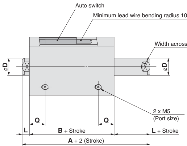
Rod end male thread
