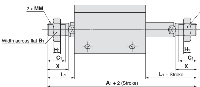
Rod end male thread
