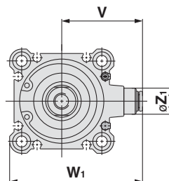
Cylinder tube form Ø63
