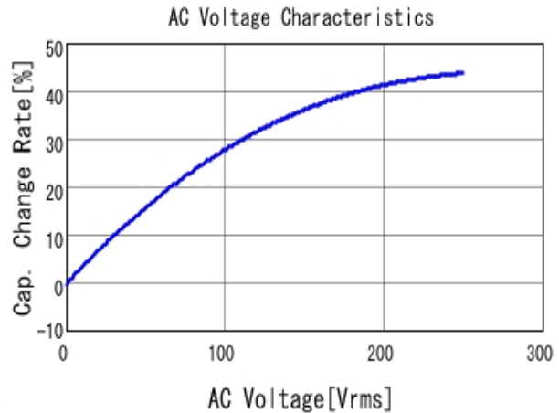
■ DE2E3KY102MB2BM01F C-AC Voltage capchange, DCOV, 20.0
