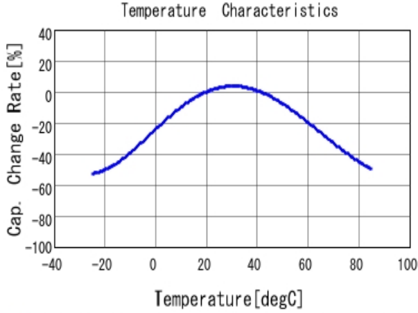
■ DE2E3KY102MB2BM01F C-Temp. capchange, DCOV, AC1Vrms
