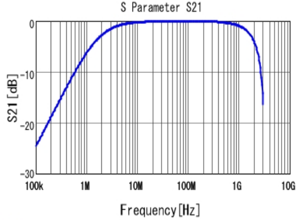
■ DE2E3KY102MB2BM01F S21 DCOV, 20degC
