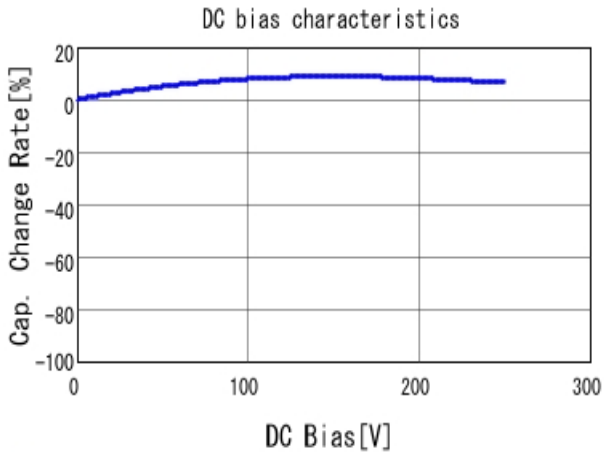
■ DE2E3KY102MA2BM01F C-DC bias capchange, 20.0degC, AC1
