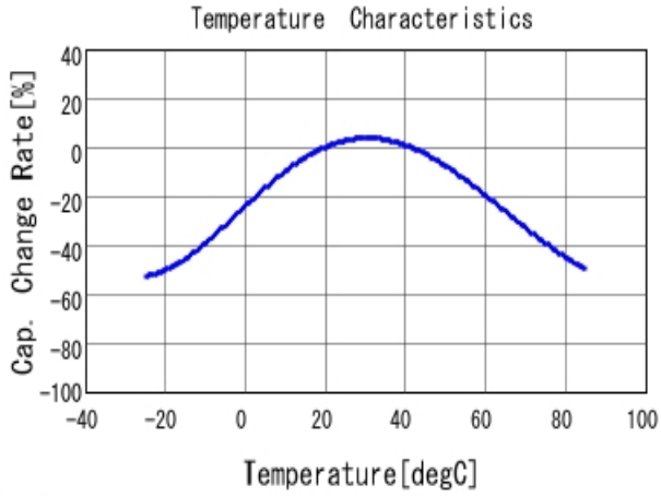
■ DE2E3KY102MA2BM01F C-Temp. capchange, DCOV, AC1Vrms
