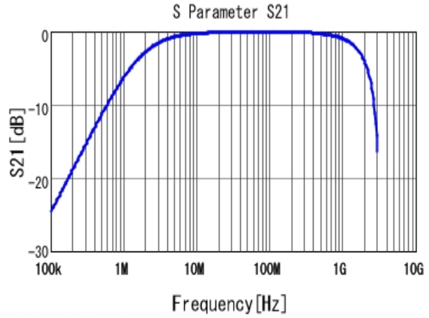
■ DE2E3KY102MA2BM01F S21 DCOV, 20degC
