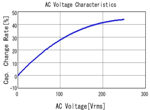
■ DE2E3KY102MA2BM01F C-AC Voltage capchange, DCOV, 20.0
