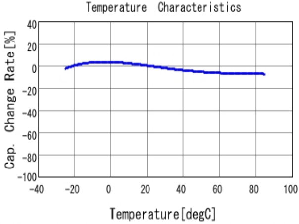
■ DE2B3KY471KA2BM01F C-Temp. capchange, DCOV, AC1Vrms
