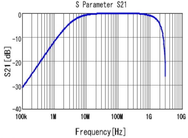
■ DE2B3KY471KA2BM01F S21 DCOV, 20degC
