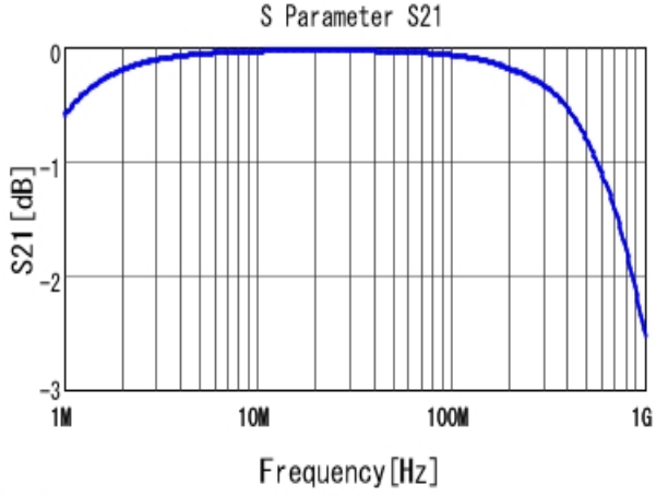
■ DE1E3RA472MA4BN01F S21 DCOV, 20degC
