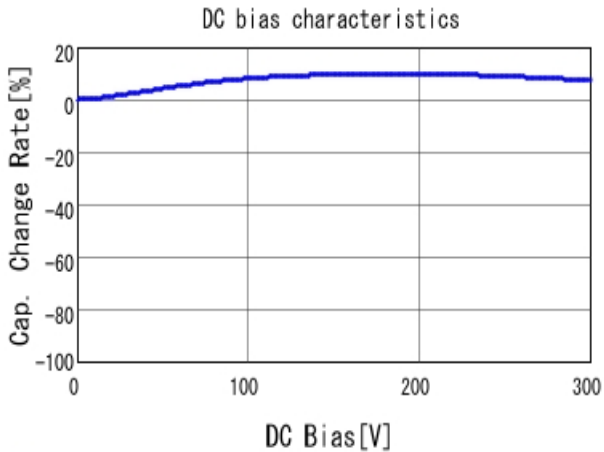
■ DE1E3KX472MN4AP01F C-DC bias capchange, 20.0degC, AC1
