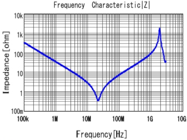
■ DE1E3KX472MN4AP01F |Z| DC0V, 20degC
