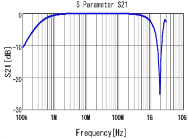
■ DE1E3KX472MN4AP01F S21 DCOV, 20degC
