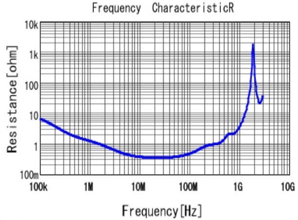
■ DE1E3KX472MN4AP01F R DC0V, 20degC
