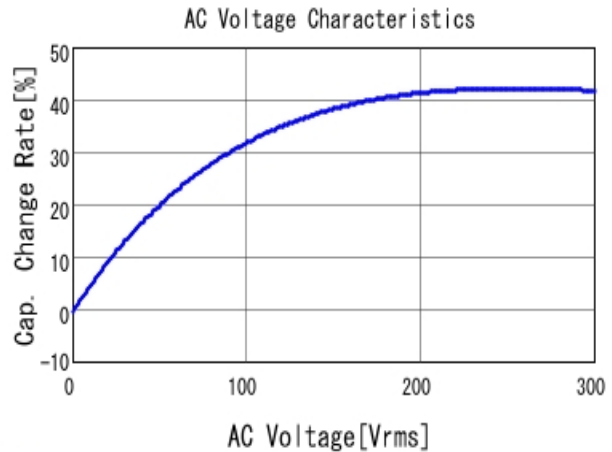
■ DE1E3KX472MN4AP01F C-AC Voltage capchange, DC0V, 20.0
