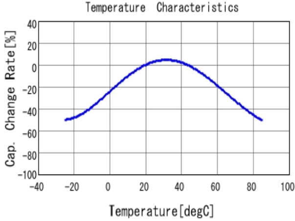
■ DE1E3KX472MN4AP01F C-Temp. capchange, DCOV, AC1Vrms
