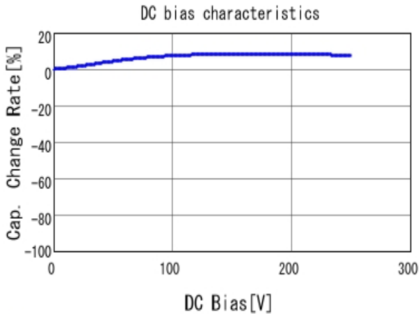
■ DE1E3KX222MA4BN01F C-DC bias capchange, 20.0degC, AC1
