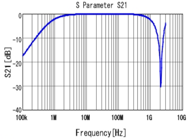
■ DE1E3KX222MA4BN01F S21 DCOV, 20degC
