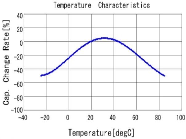
■ DE1E3KX222MA4BN01F C-Temp. capchange, DCOV, AC1Vrms
