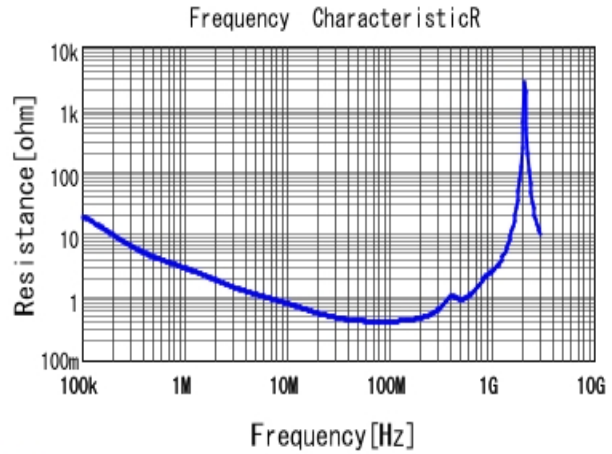
■ DE1E3KX222MA4BN01F R DC0V, 20degC
