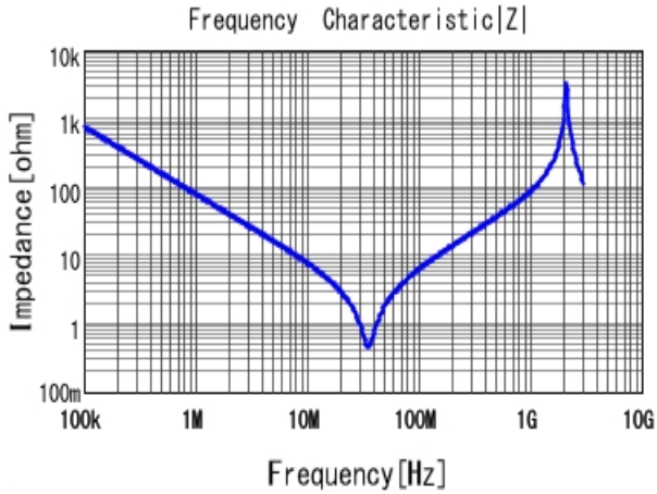
■ DE1E3KX222MA4BN01F |Z| DC0V, 20degC
