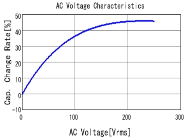
■ DE1E3KX222MA4BN01F C-AC Voltage capchange, DC0V, 20.0
