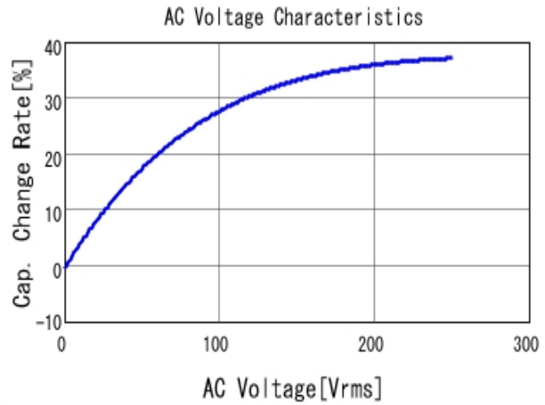
■ DE1E3KX102MN4AN01F C-AC Voltage capchange, DCOV, 20.0
