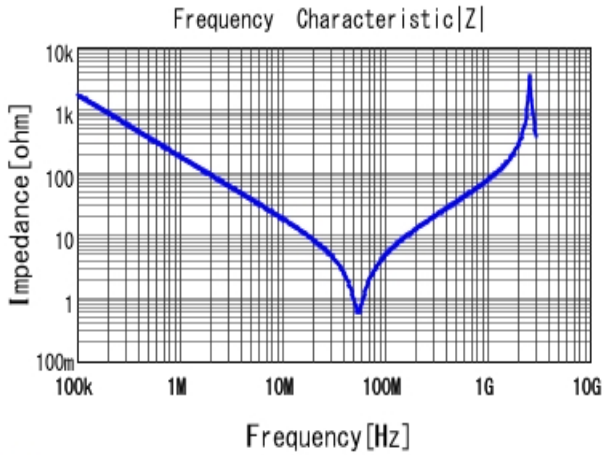
■ DE1E3KX102MN4AN01F |Z| DCOV, 20degC
