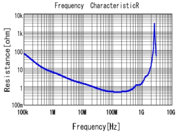
■ DE1E3KX102MN4AN01F R DCOV, 20degC
