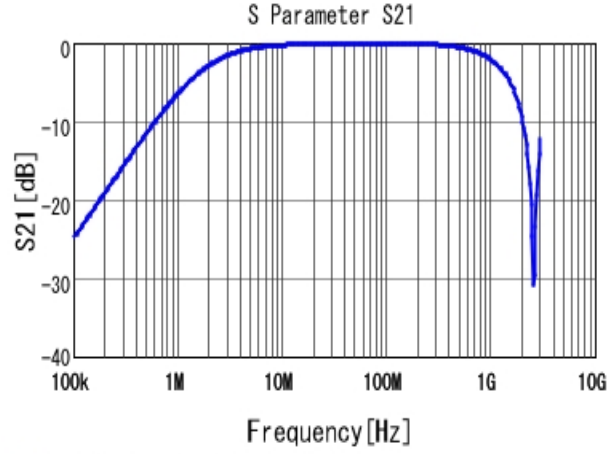
■ DE1E3KX102MN4AN01F S21 DCOV, 20degC
