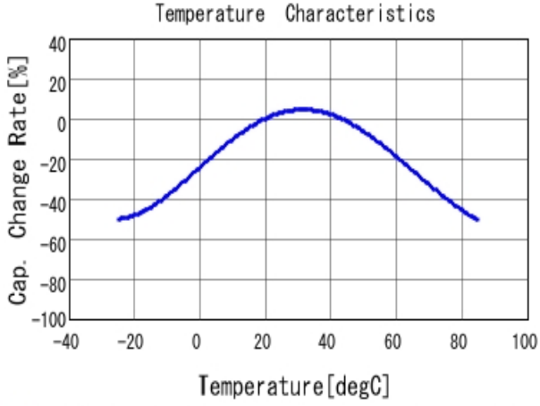
■ DE1E3KX102MN4AN01F C-Temp. capchange, DCOV, AC1Vrms
