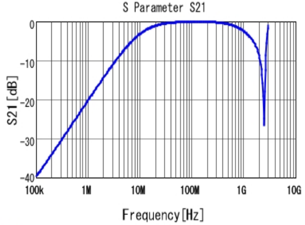
■ DE1B3KX221KA4BN01F S21 DCOV, 20degC
