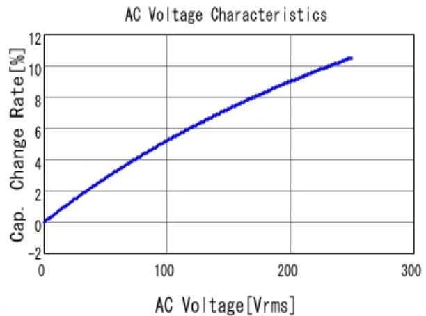
■ DE1B3KX221KA4BN01F C-AC Voltage capchange, DCOV, 20.0
