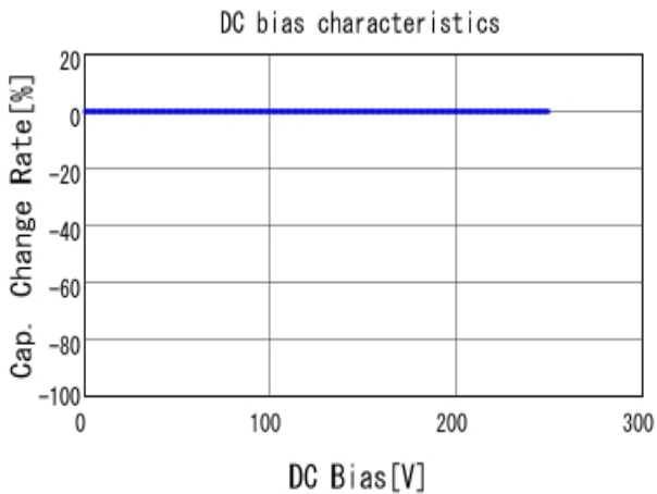
■ DE1B3KX221KA4BN01F C-DC bias capchange, 20.0degC, AC1
