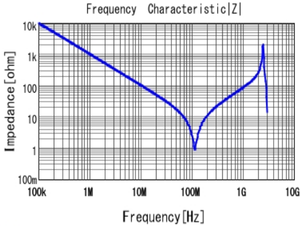
■ DE1B3KX221KA4BN01F |Z| DCOV, 20degC
