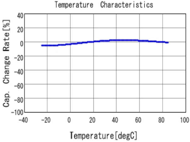
■ DE1B3KX221KA4BN01F C-Temp. capchange, DCOV, AC1Vrms
