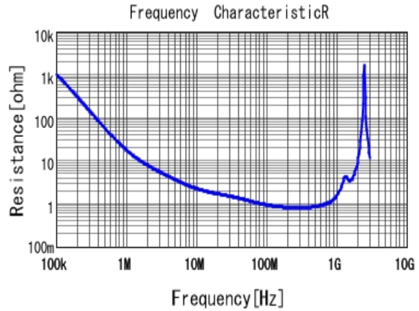
■ DE1B3KX221KA4BN01F R DCOV, 20degC
