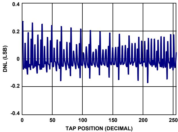
FIGURE 3. 10k DNL vs TAP POSITION, V CC = 5V
