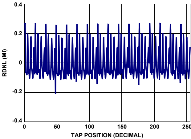
FIGURE 7. 10k RDNL vs TAP POSITION, V CC = 5V
