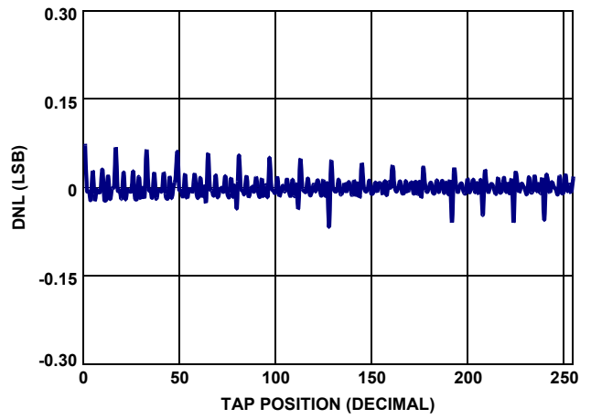
FIGURE 4. 50k DNL vs TAP POSITION, V CC = 5V
