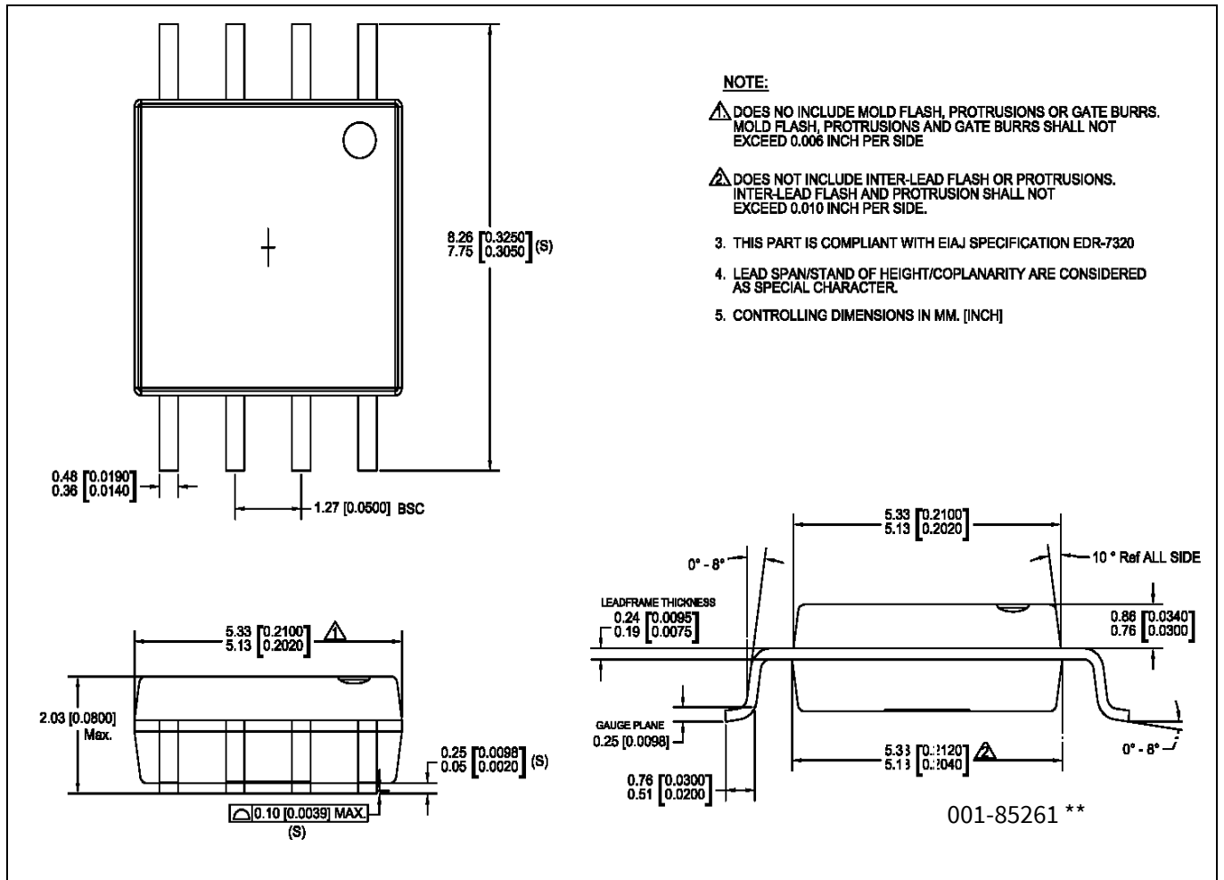
Figure 26 8-pin SOIC (208 Mils) package outline, 001-85261
