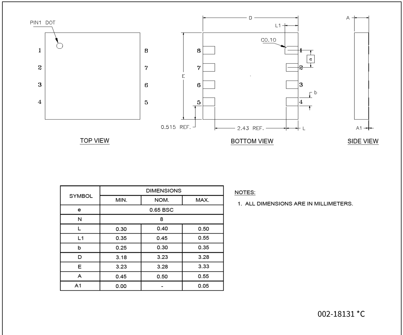
Figure 27 8-pin GQFN (3.23 × 3.28 × 0.55 mm) package outline, 002-18131
