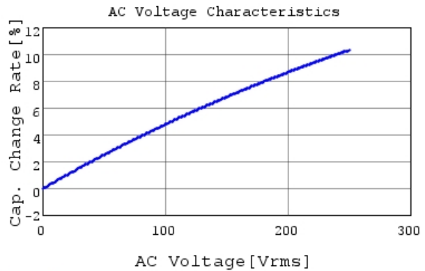
DE1B3KX101KA4BN01F C-AC Voltage capchange, I
