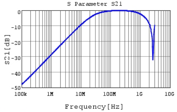
DE1B3KX101KA4BN01F S21 DCOV, 20degC
