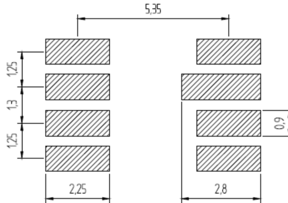
Figure 21: MS5803-07BA recommended pad layout
