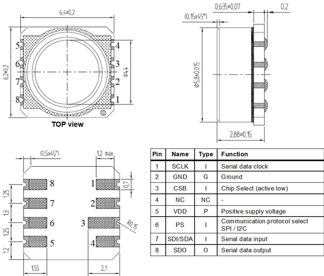
Figure 20: MS5803-07BA package outlines, pin configuration and description
