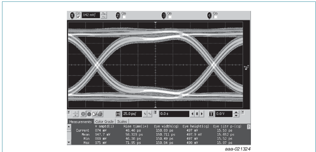
Fig 6. HDMI 2.0 eye diagram TP1, test board with PESD3USB30; typical values
