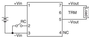
Connection diagram
