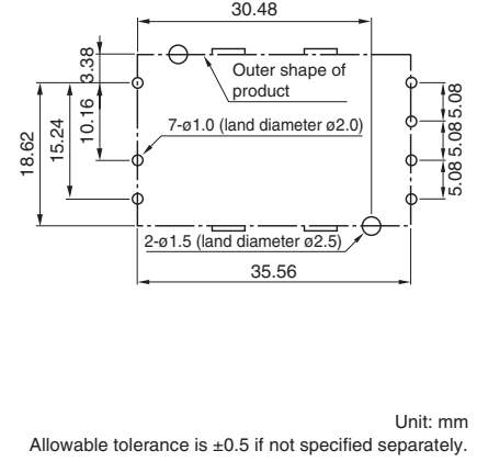
Recommended measurements for mounting board
