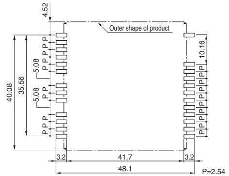
Recommended measurements for mounting board
