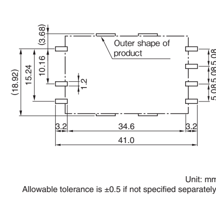
Recommended measurements for mounting board
