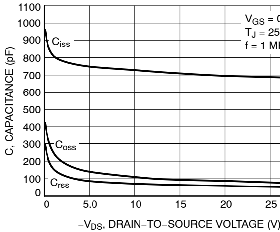
Figure 7. Capacitance Variation
