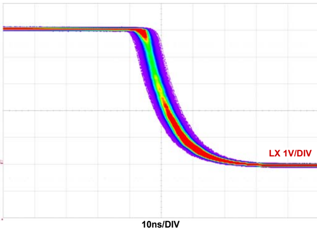
FIGURE 41. JITTER AT NO LOAD F_{SW} = 2\text{MHz} , V_{IN} = 5\text{V} , MODE = PWM, T_A = +25^\circ\text{C}
