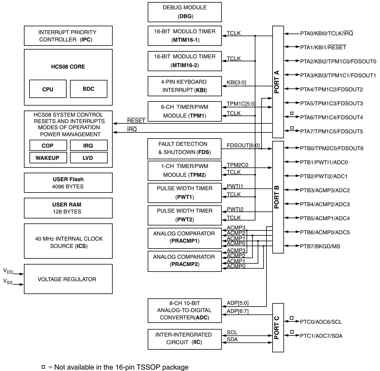
Figure 1. MC9S08SF4 Series Block Diagram
