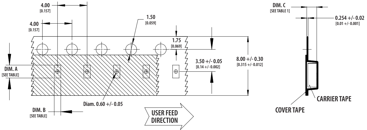
Figure 8. Tape Dimensions.
