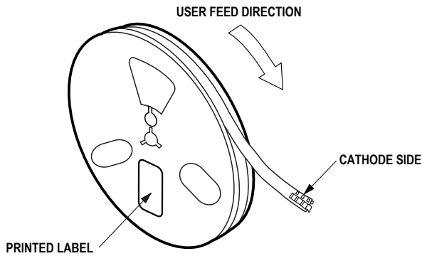
Figure 9. Reeling Orientation.
