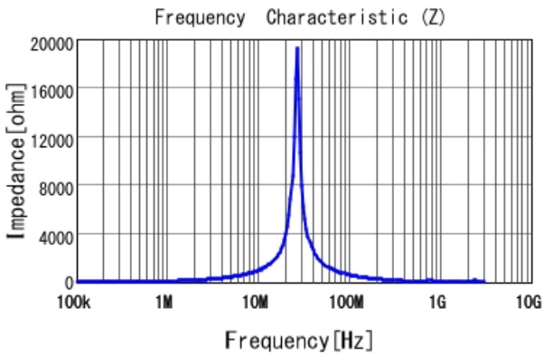
■ LQH5BPN150MT0 |Z|
