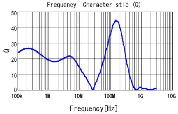
■ LQH5BPN150MT0 Q
