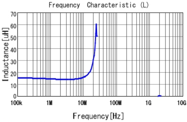
■ LQH5BPN150MT0 L
