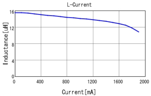
■ LQH5BPN150MT0 L-Current 20degC
