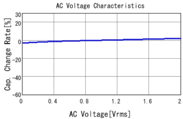
GRM155R71H102KA01 C-AC Voltage capchange, DCOV, 25
