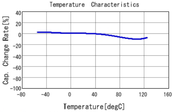
GRM155R71H102KA01 C-Temp. capchange, DC0.0V, AC1.C
