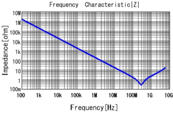
GRM155R71H102KA01 |Z| DCOV, 25degC
