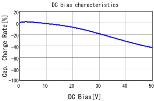
GRM155R71H102KA01 C-DC bias capchange, 25.0degC, A
