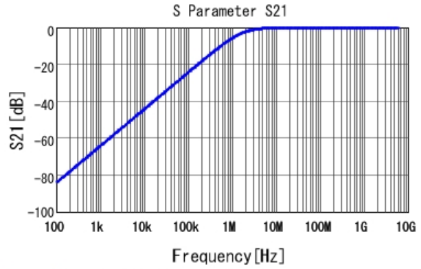
GRM155R71H102KA01 S21 DC0V, 25degC
