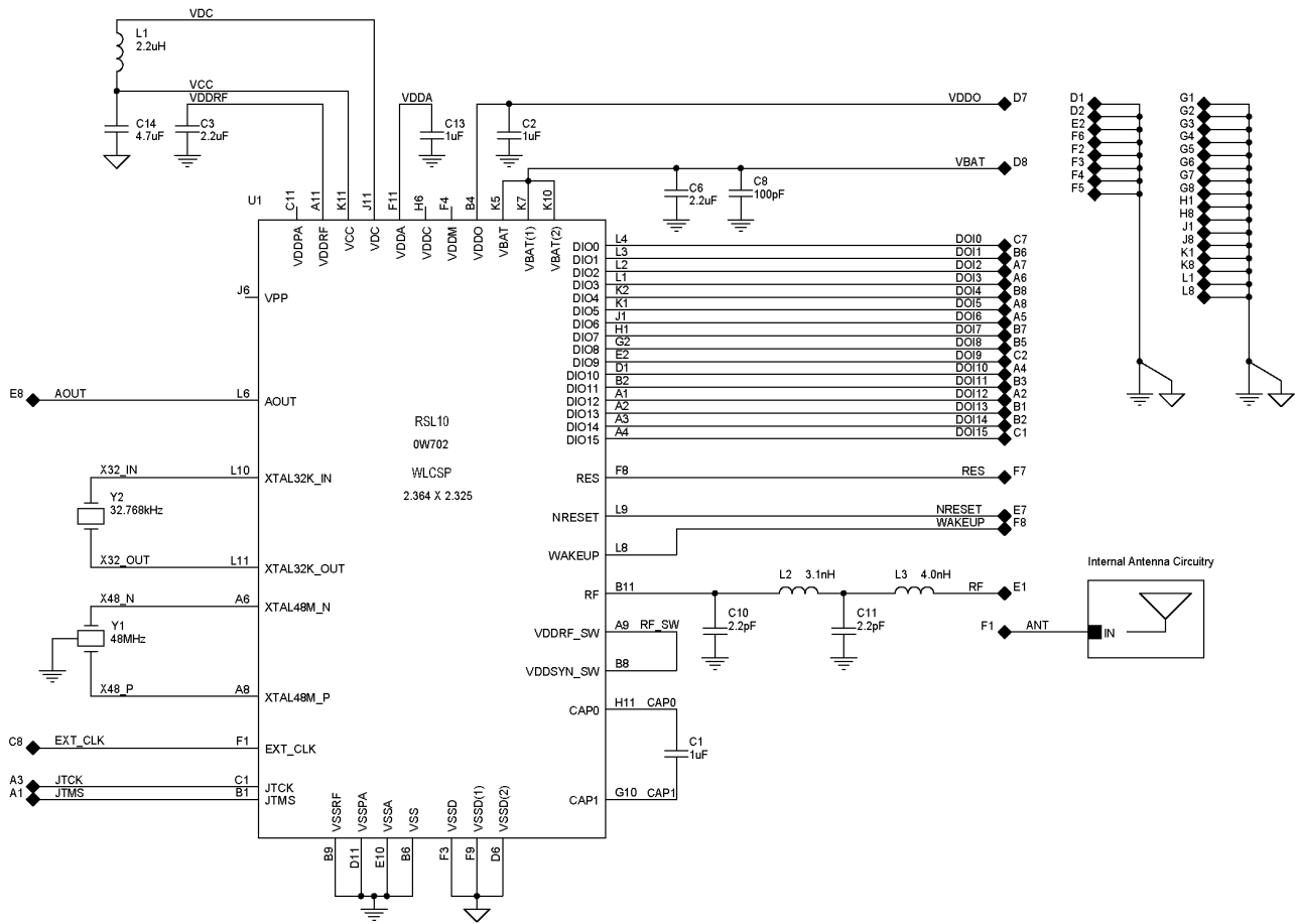
Figure 3. RSL10 SIP Schematic
