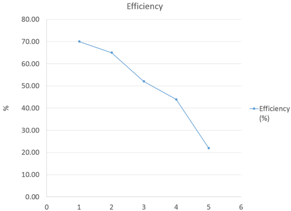
Figure 5. Antenna Efficiency vs. PCB Size.
