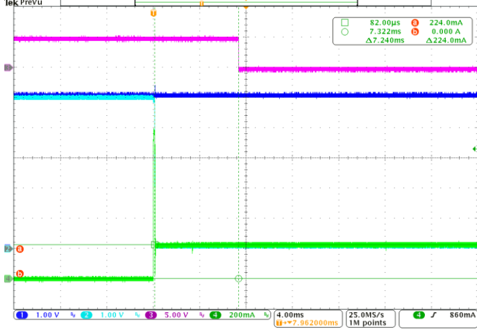
Overcurrent Limit Response
