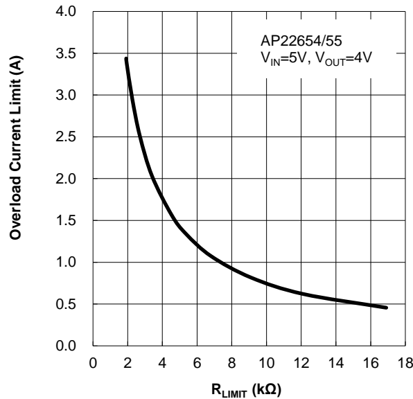
Figure 2. R_{LIMIT} vs. Overload Current Limit
